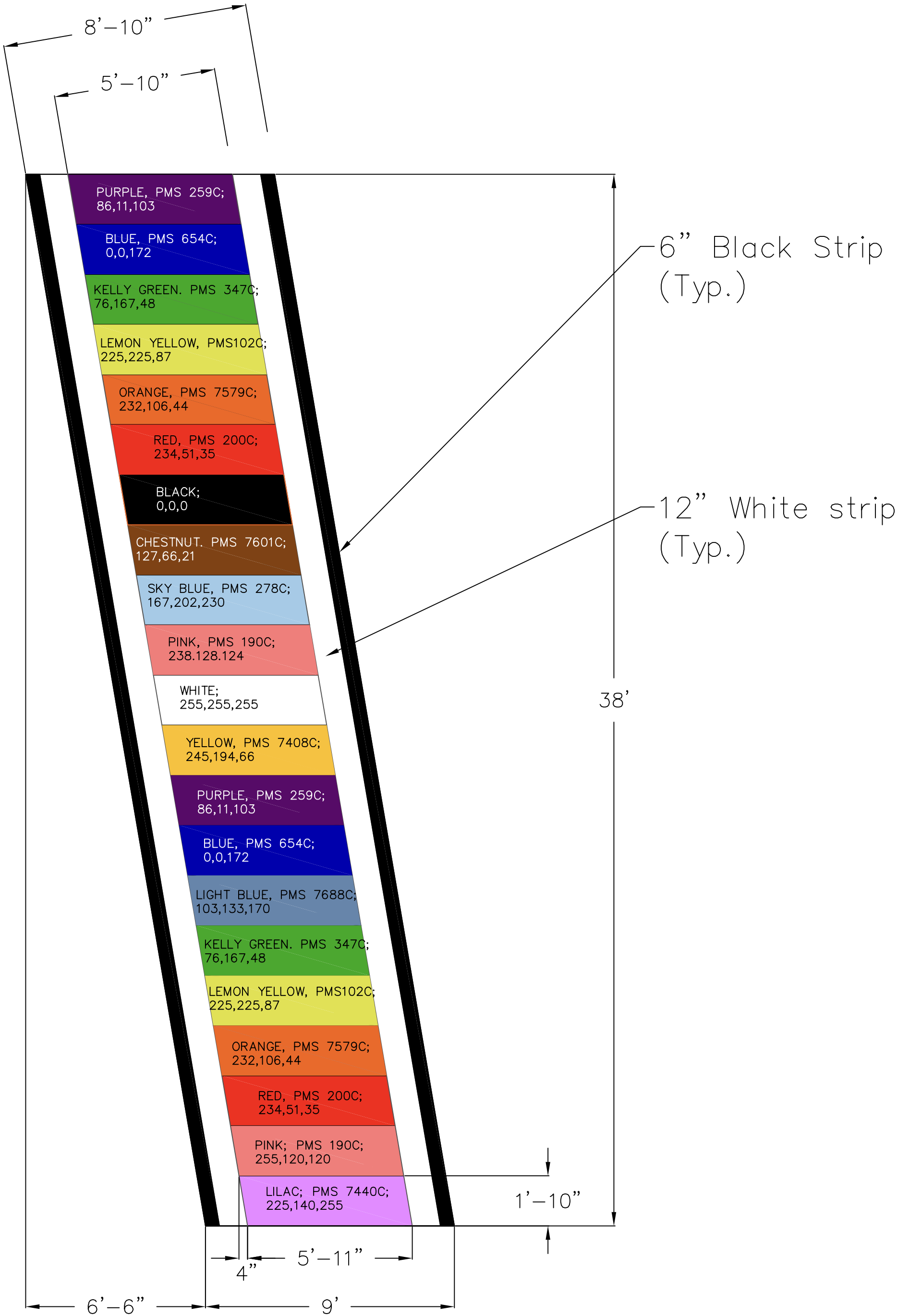
PROPOSED RAINBOW CROSSWALK JESUP RD & TAYLOR PLACE WESTPORT, CT WESTPORT ENGINEERING DIVISION
